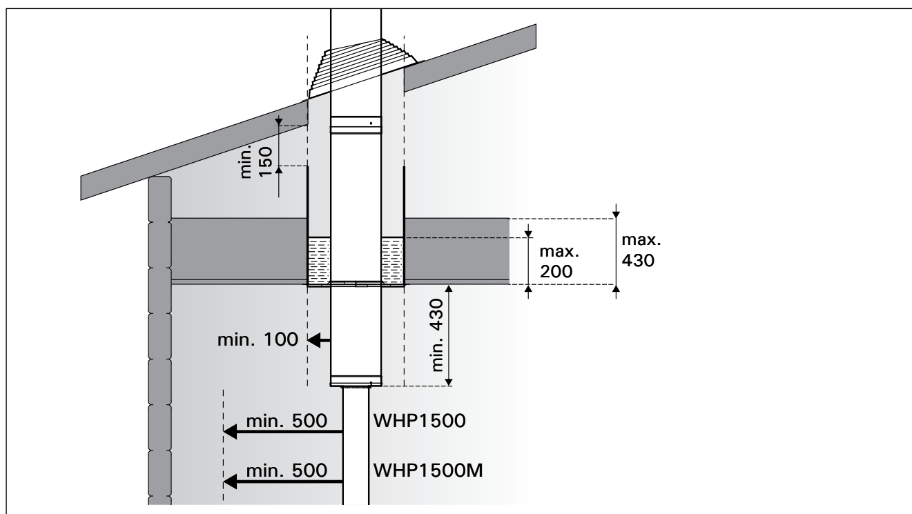
Figure 2. Safety distances (all dimensions in millimeters)
